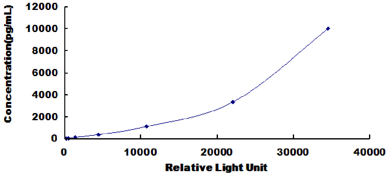
Typical Standard Curve for Mouse MUC5AC CLIA.
